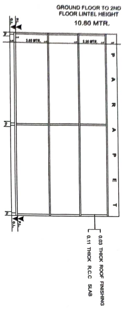
SECTION AT A-B
